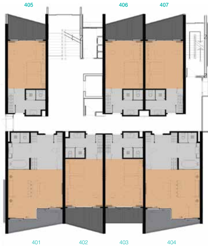
4 th FLOOR PLAN
