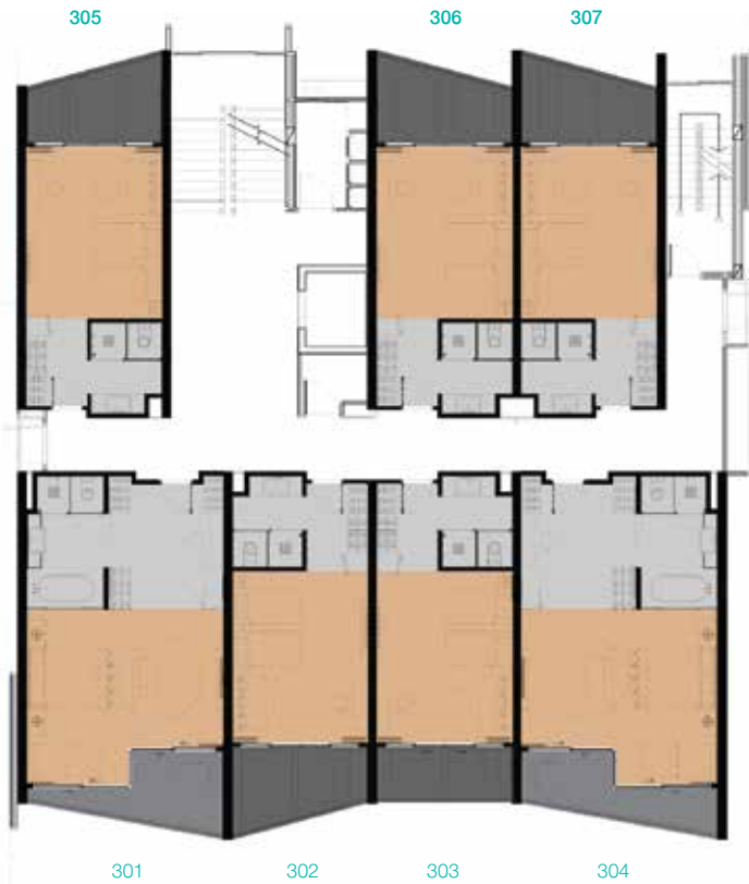
3 rd FLOOR PLAN
